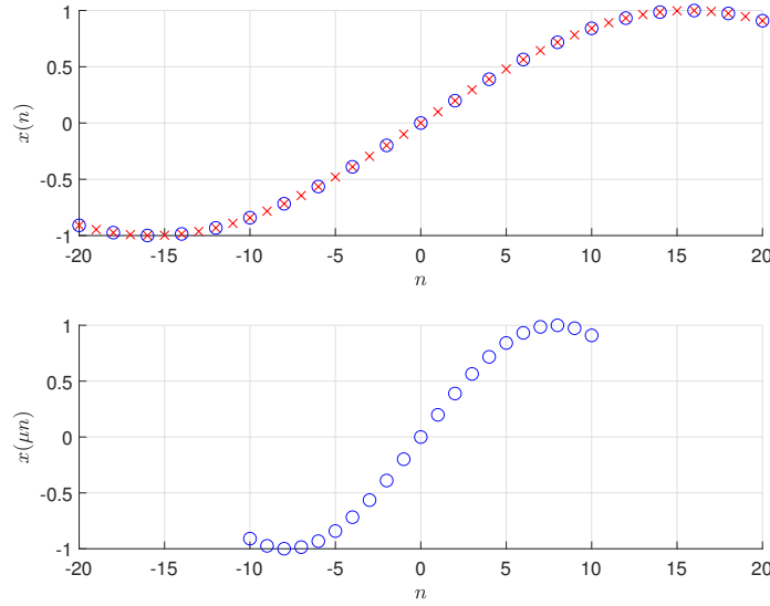
FIGURE 3.4: A demonstration of down-sampling.
