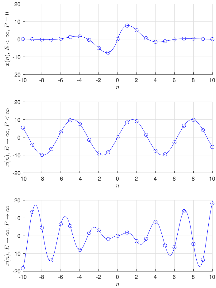
FIGURE 3.3: Example of energy and power signals.
