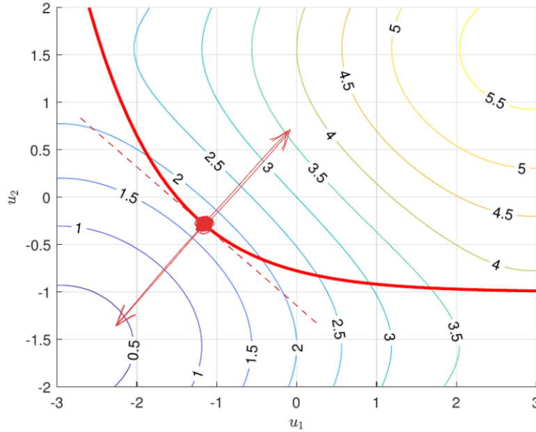
FIGURE 5.2: Graphical explanation to (5.9).
