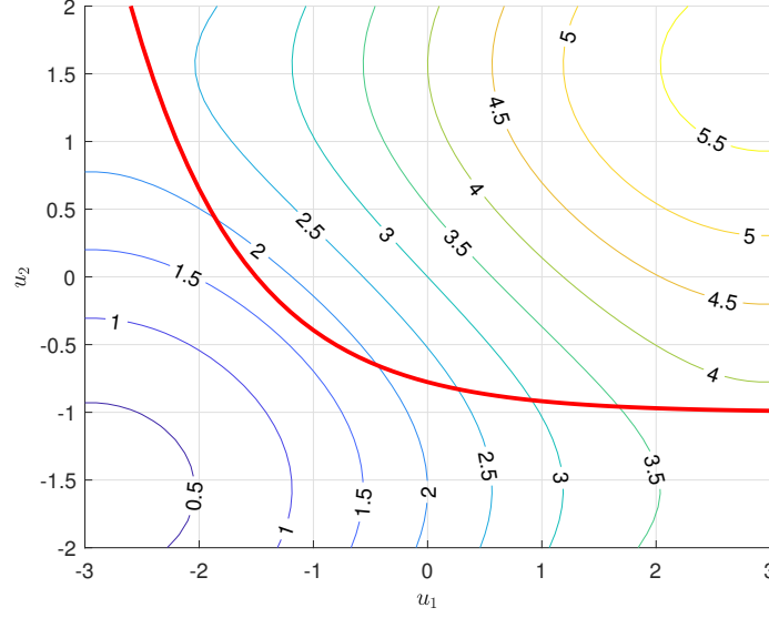
FIGURE 5.1: Static optimization with equality constraint demonstration.
